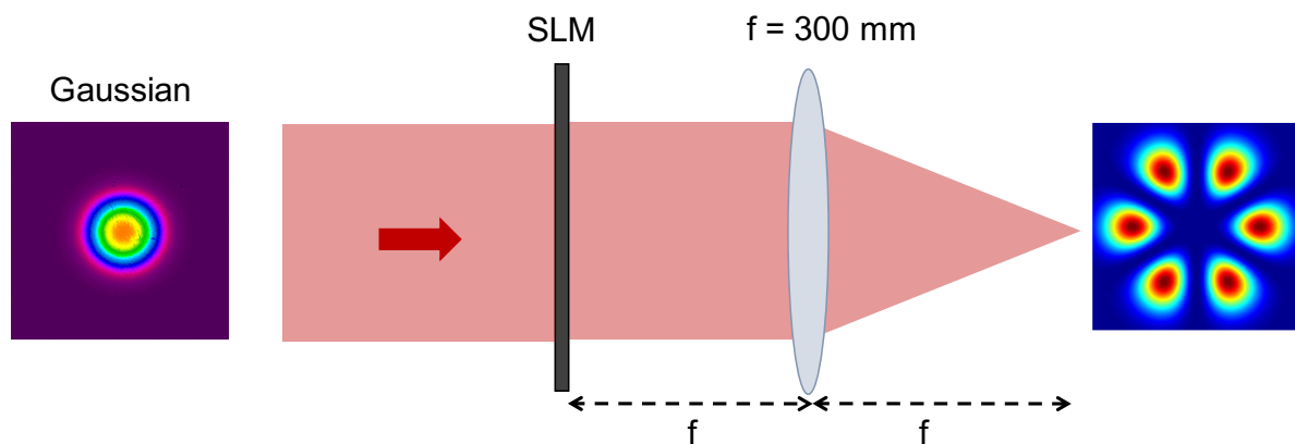
Figure 1: The laboratory set-up with the desired mode set to the created shown in the far-field plane of the SLM.
